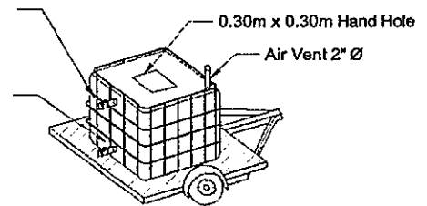
DETACHABLE SEPTIC VAULT DETAIL SCALE: NTS
